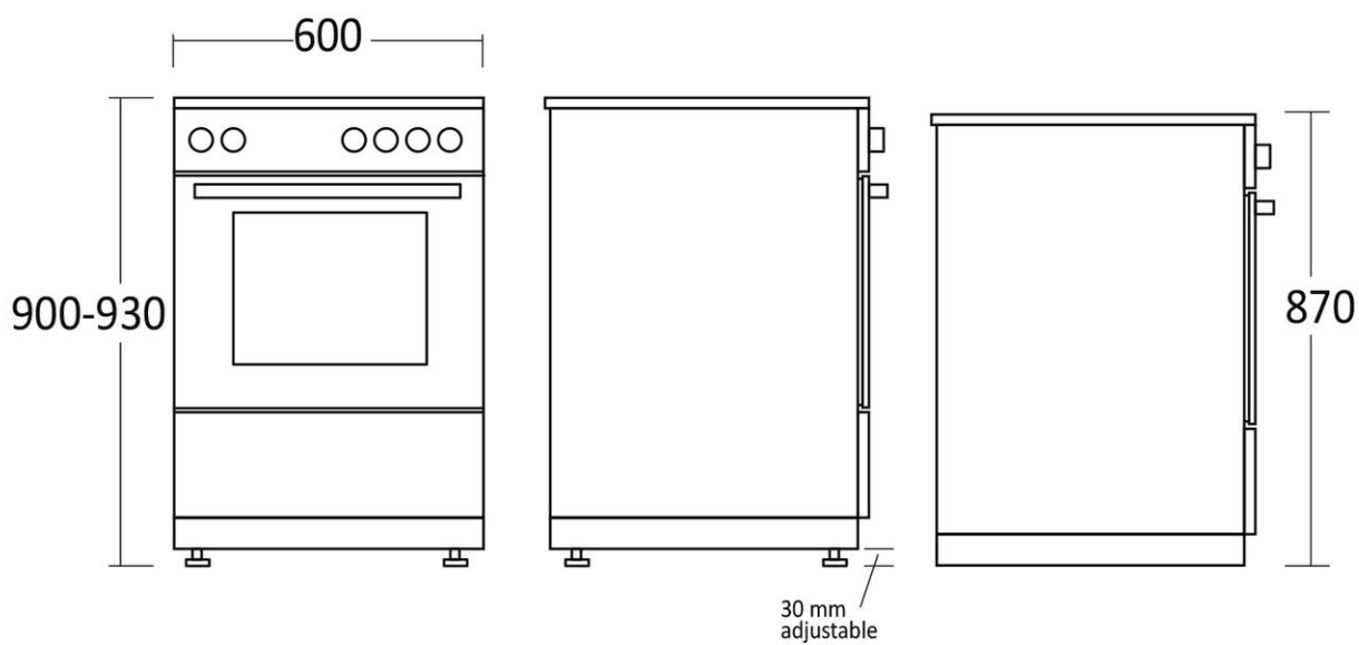
With bottom frame
