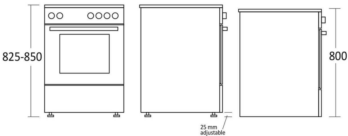
Without bottom frame
