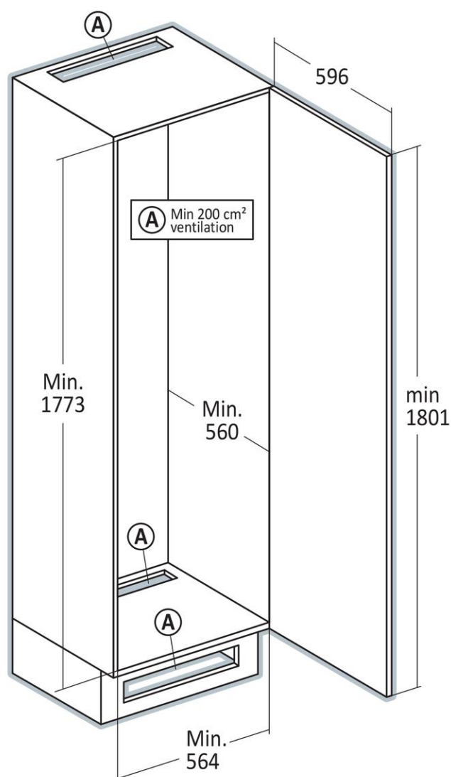
Kitchen cupboard
