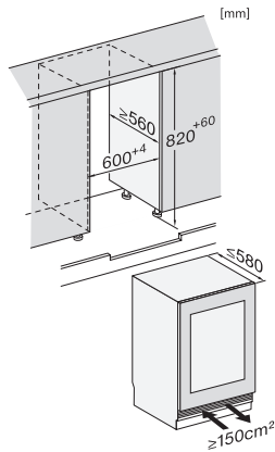
KWTUS7054F, KWTUS7055F, KWTUS7074F, KWTUS7096E, Built-under, niche dimensions
