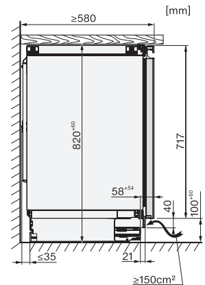
KWTUS7054F, KWTUS7055F, KWTUS7074F, Built- under, side view
